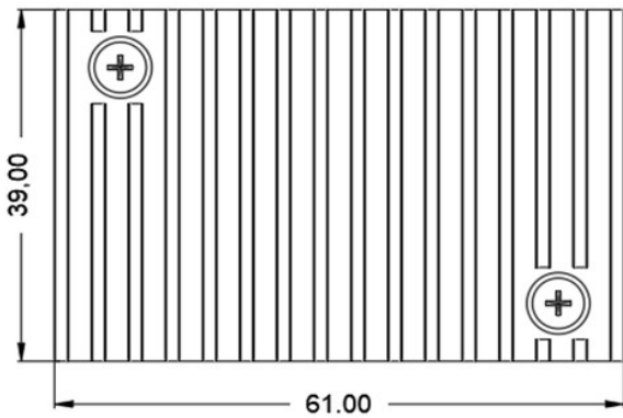
Standard+Heatsink 61.0x39.0x27.7mm
